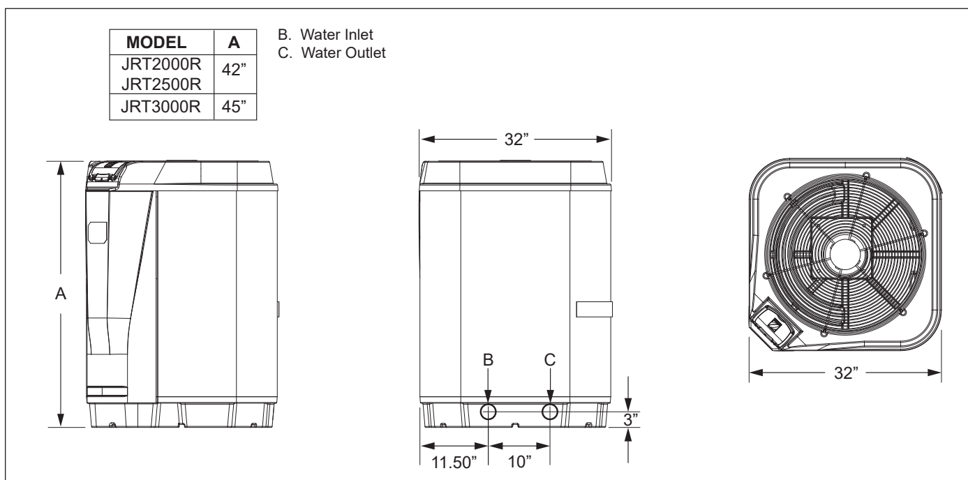
Figure 1. Jandy JRT Heat Pumps Dimensions
