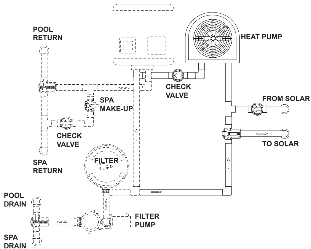
Figure 5. Plumbing For Heating System Combinations
