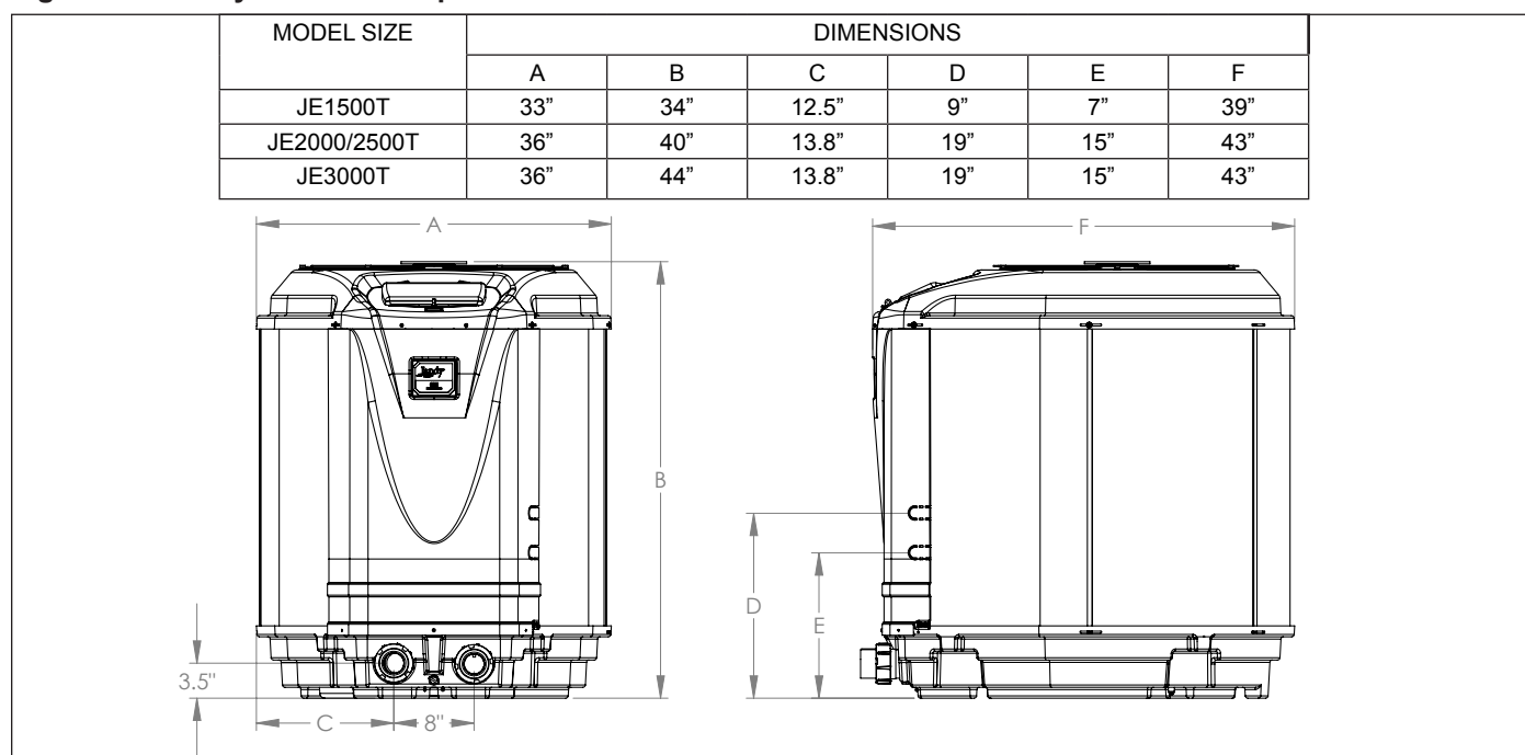
Figure 1. Jandy JE Heat Pumps Dimensions
