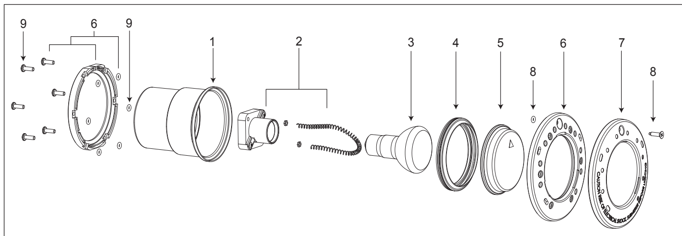
Figure 12. Jandy Spa White Light Exploded View
