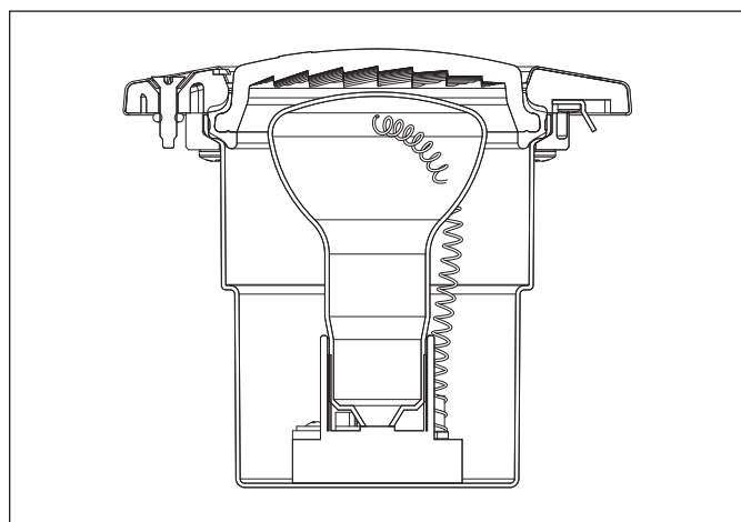
Figure 14. Cross Section of Jandy Spa White Light
