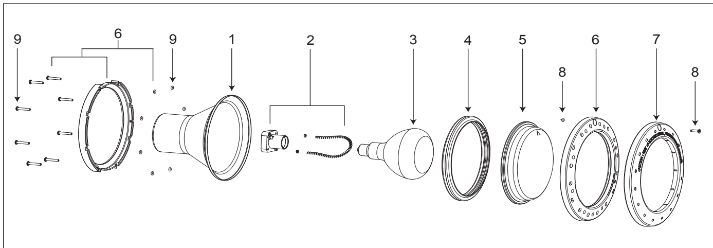
Figure 9. Jandy Pool White Light Exploded View
