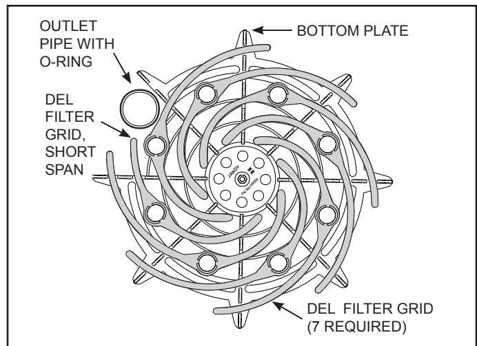
Figure 9. Filter Grid Arrangement
